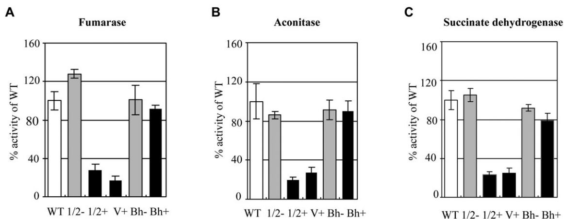
Fig. 7. Biochemical consequences of TbIsa1/2 double knock-down rescued with B. hominis Isa2 proteins in PF T. brucei . Enzymatic activities of fumarase (A), aconitase (B) and succinate dehydrogenase (C) were measured in the digitonin isolated mitochondria. A given activity in 29–13 PF cells represents 100% (white column). Activity in non-induced TbIsa1/2 cells (1/2–) and the same cell transfected with BhIsa2 (Bh–) is shown in grey columns. Activity in RNAi-induced TbIsa1/2 (1/2+), TbIsa1/2 with an empty pABPURO vector (V+), and those transfected with BhIsa2 (Bh+) after 4 days of RNAi induction is shown in black columns; the mean and the SD values represent the average of measurements from three independent RNAi induction.
