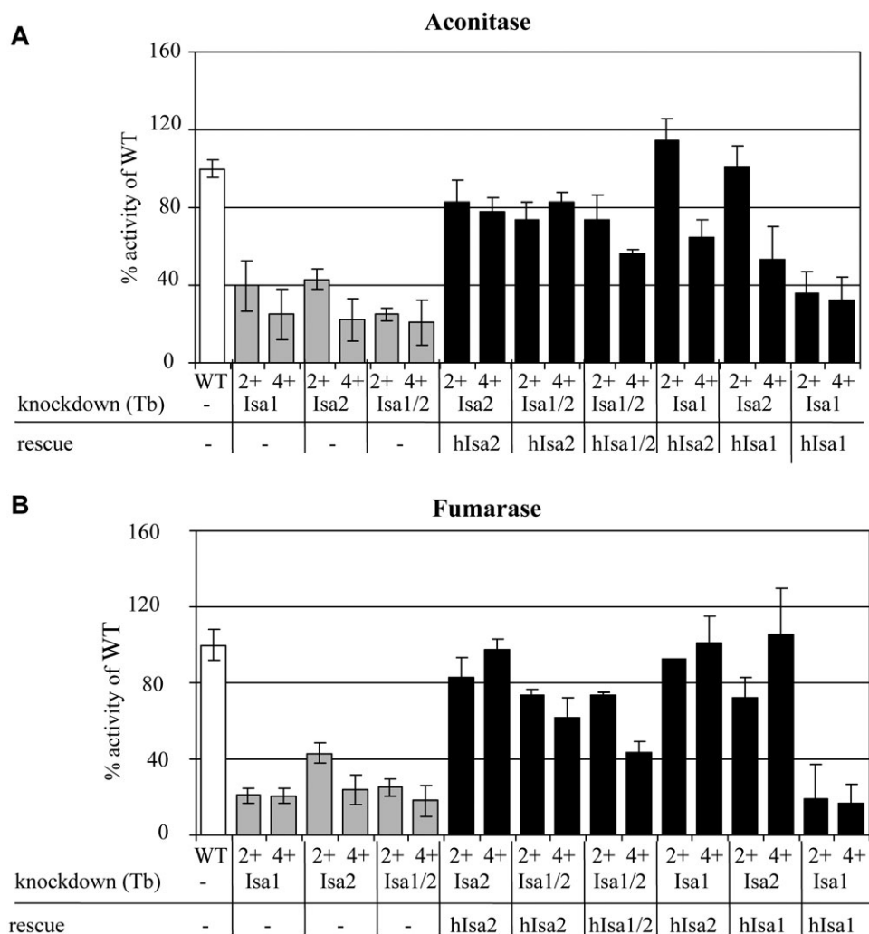
Fig. 6. Biochemical consequences of Tblsa knock-downs (cross) rescued with human Isa proteins in PF T. brucei .
