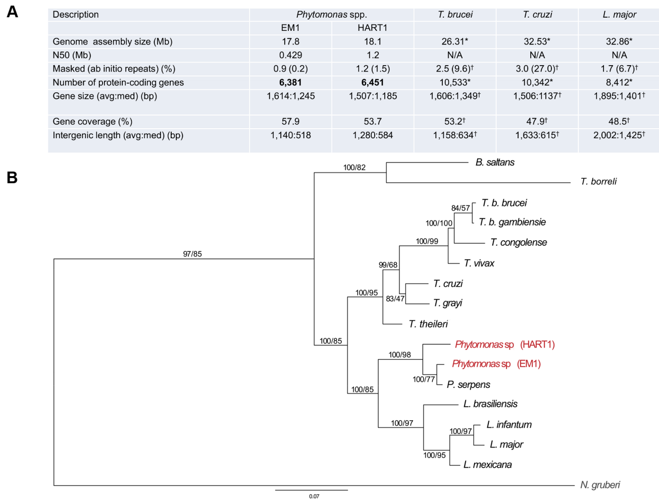
Figure 1. General features of Phytomonas EM1 and HART1 isolates. A. Statistics on Phytomonas EM1 and HART1 genome annotations. Results of both Phytomonas genome annotations, together with statistics on T. brucei TRE927 ( T. brucei ), T. cruzi CL Brener Esmeraldo-like ( T. cruzi ) and L. major Friedlin ( L. major ) genome annotations, either obtained by directly querying the TriTrypDB release 4.2 (*) or by using the same analysis pipeline applied for both Phytomonas spp. ( † ), are summarized; B. Phylogenetic reconstruction of HSP90 evolution in the trypanosomatids. HSP90 sequence data are taken from [127], together with the top BLAST hits retrieved from HART1 and EM1 genome sequence data using HSP90 as a query. Orthology was established by reverse BLAST into the non-redundant database. Trees were constructed by multiple sequence alignment followed by trimming of the N- and C-termini (the EM1 sequence is truncated), and reconstructions by Mr Bayes and PhyML. Statistical support is shown for all nodes as Mr Bayes/PhyML posterior probabilities/bootstraps, respectively. The two Phytomonas isolates analysed here are colored in red, and the N. gruberi sequence, included as an outgroup, is in gray. Note that branch lengths indicate that EM1 and HART1 are of similar divergence as T. brucei versus T. congolense or L. infantum versus L. mexicana . EM1 is more closely related to P. serpens than to HART1 based on this dataset. doi:10.1371/journal.pgen.1004007.g001
