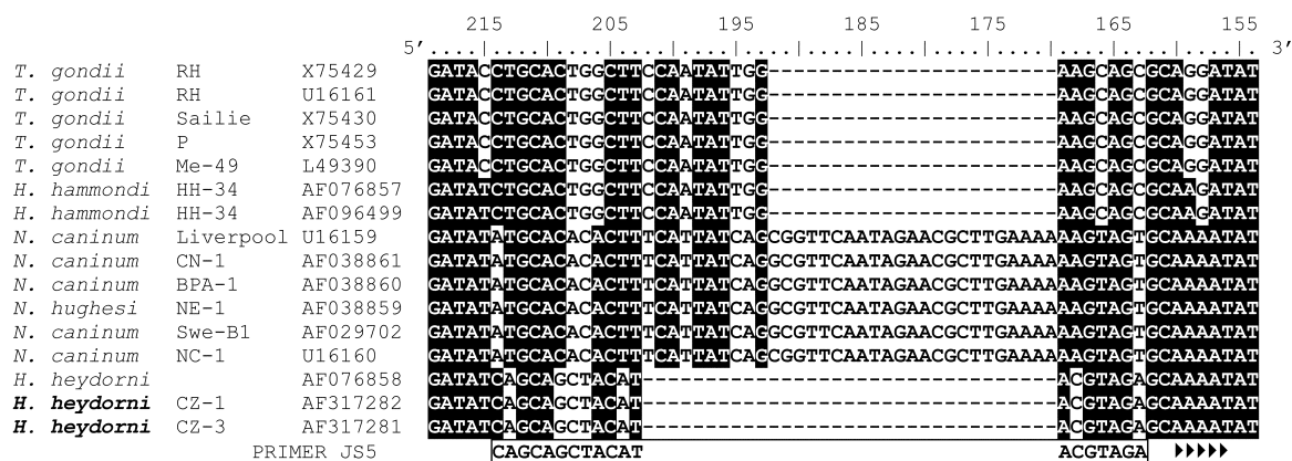
Fig. 2. Clustal X generated partial alignment of positions 154–219 of ITS1 sequences of closely related species; species, strain/isolate and GenBank accession nos. are given on the left; sequences obtained in this study are in bold; JS5 primer is marked below, arrows show the direction of the primer toward the SSU rRNA gene.
