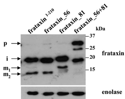
Fig. 6. Processing of mutated frataxin in T. brucei . Western analysis of total lysates of the T. brucei Tb-frataxin RNAi knockdown cells stably expressing frataxin 1-210 (frataxin 1-210 ), frataxin 1-210 with mutated processing site 56 (frataxin 56 ), frataxin 1-210 with mutated processing site 81 (frataxin 81 ), and frataxin 1-210 with mutated processing sites 56 and 81 (frataxin 56+81 ). The labeling of p, i, m 1 and m 2 as in Figs. 1 and 3. \alpha -Enolase antibodies were used as a loading control.
