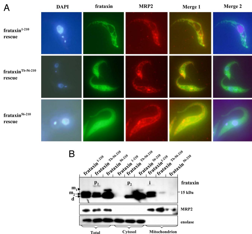
Fig. 4. Mitochondrial localization of frataxin in rescued cell lines. (A) Immunolocalization of frataxin. Cells stably expressing frataxin 1-210 , frataxin Tb-56-210 , or frataxin 56-210 were fixed and treated with \alpha -frataxin mouse monoclonal antibody and \alpha -MRP2 rabbit polyclonal antibody, followed by donkey \alpha -mouse antibody (green) and donkey \alpha -rabbit antibody (red). Finally, the cells were stained with DAPI. The merged images show complete (frataxin 1-210 ), partial (frataxin Tb-56-210 ), and lack of co-localization (frataxin 56-210 ) of frataxin with the mitochondrial protein MRP2. Merge 1 is given for colocalization of frataxin with MRP2. Merge 2 is given for colocalization of frataxin and DAPI. (B) Immunoblot analysis of frataxin expression in whole-cell lysates and extracted cytosolic and mitochondrial fractions of T. brucei frataxin RNAi knockdown transfected with constitutively expressed frataxin 1-210 , frataxin Tb-56-210 , or frataxin 56-210 . MRP2 and enolase proteins were used as mitochondrial and cytosolic controls, respectively. The labeling of p 2 , i, m 1 and m 2 as in Figs. 1 and 3.
