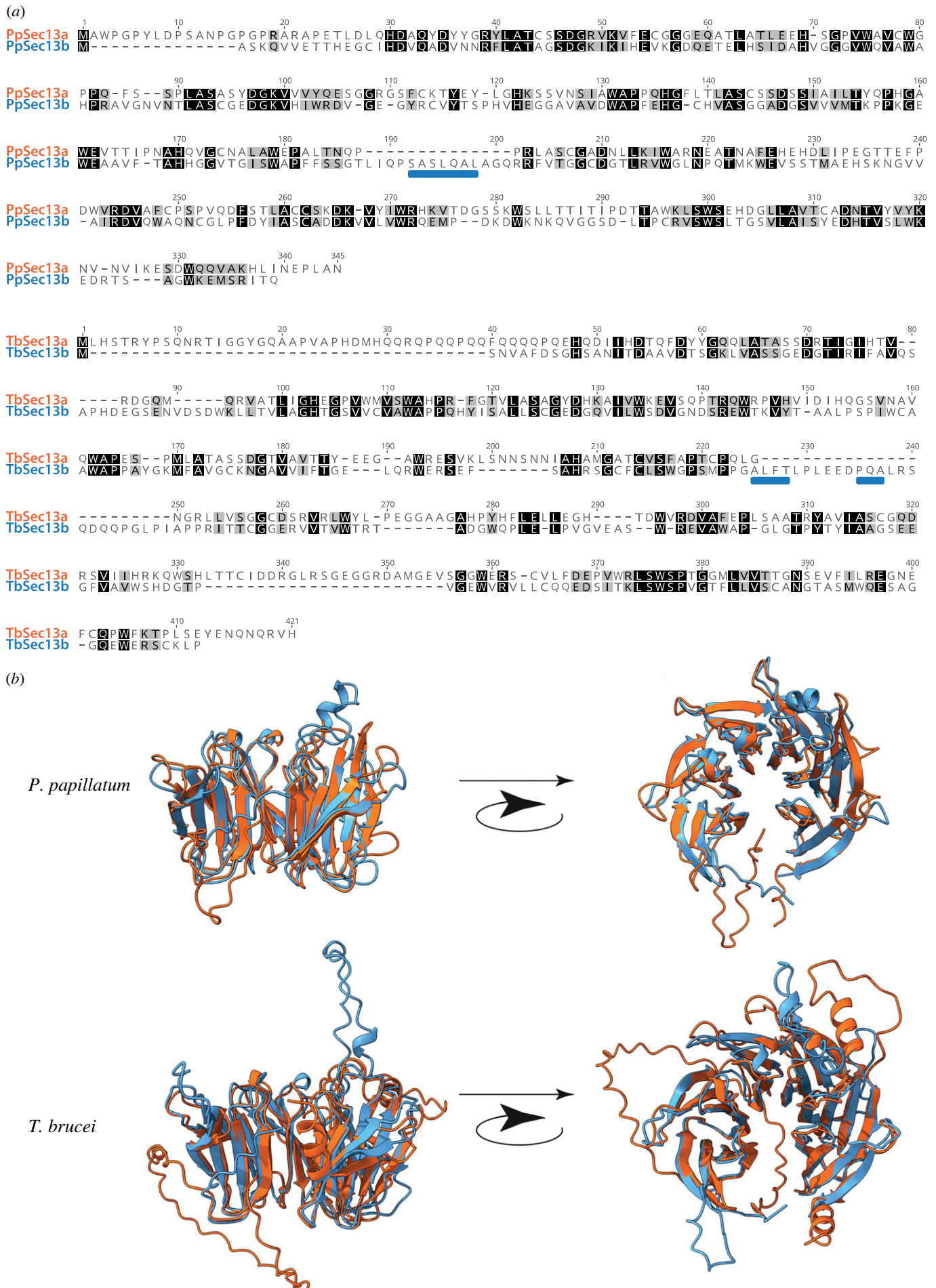
Figure 3. Structural divergence between Sec13a and Sec13b. (a) Alignments of Sec13 paralogs for P. papillatum and T. brucei . Please note that TbSec13a and TbSec13b are also named TbSec13.1 (accession number Tb927.10.14180) and TbSec13.2 (accession number Tb927.11.8120). (b) Overlaid AlphaFold predictions for Sec13a and Sec13b (colours correspond to figure 1) for P. papillatum and T. brucei to illustrate the positions of indel peptide sequences (marked by blue rectangles in (a)). Note that the positions of indels are distinct, but probably provide significantly unique binding sites to discriminate between protein interactions and hence complex association.
